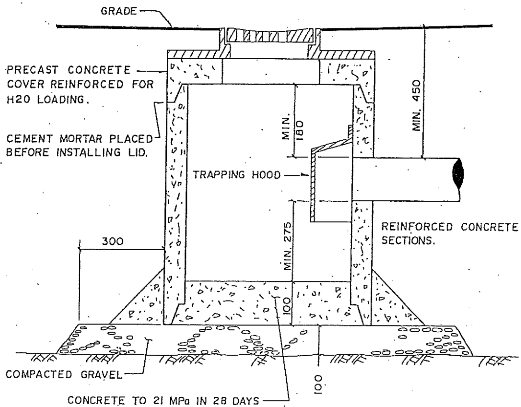
SECTION
