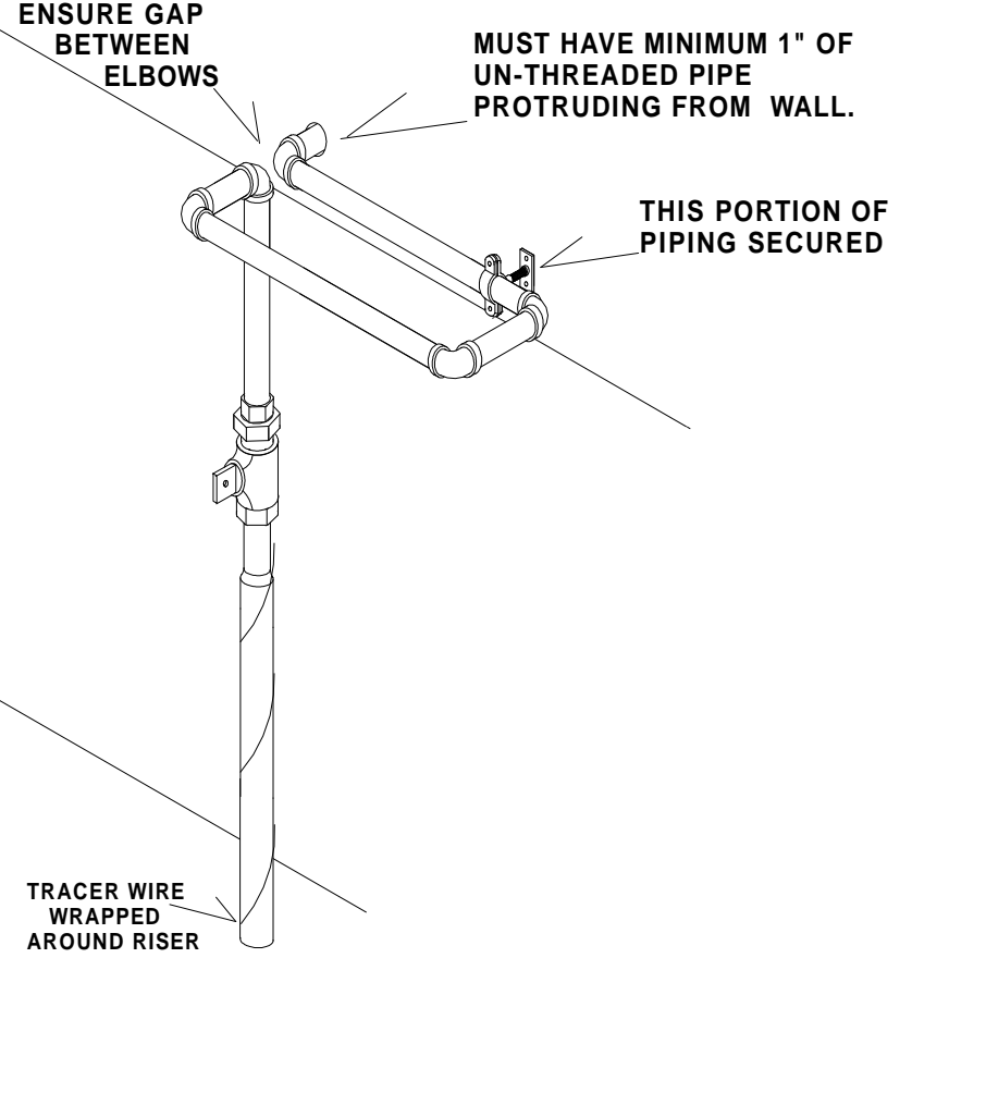
(FIG #3). Alternate Piping Configuration
