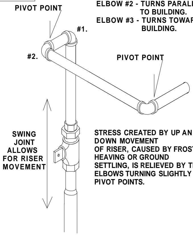
(FIG #3). Alternate Piping Configuration
