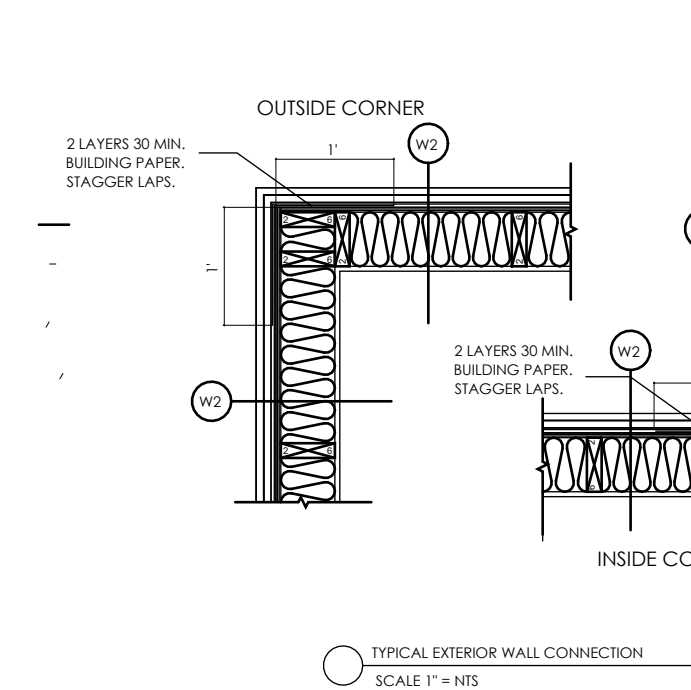
2 TYPICAL EXTERIOR WALL CONNECTION SCALE 1" = 1/4"
