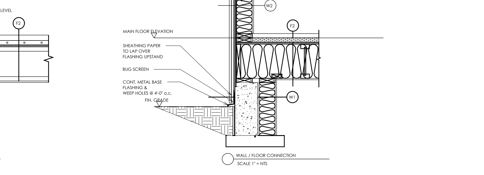
6 WALL / FLOOR CONNECTION SCALE 1" = 1/4"
