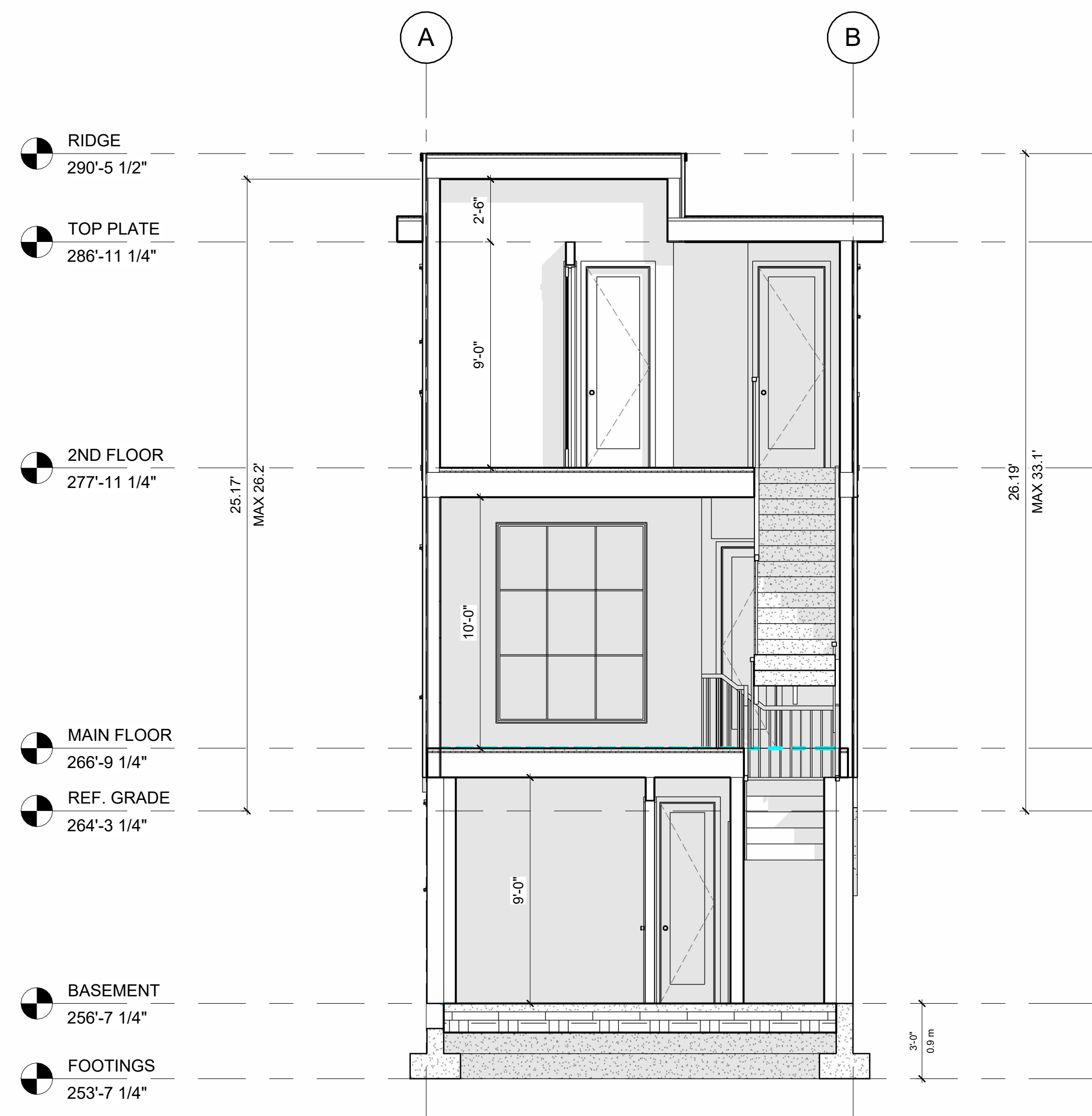
1 Section 1 1/4" = 1'-0"
