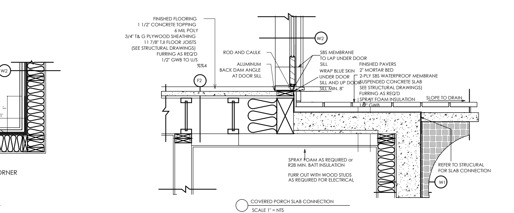
3 COVERED PORCH SLAB CONNECTION SCALE 1" = 1/4"
