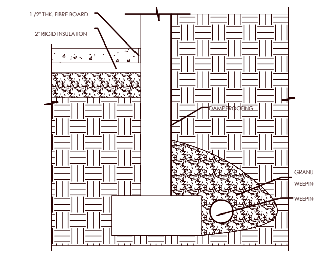
2 FOUNDATION
