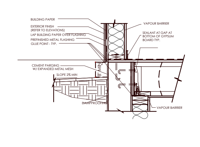
4 FLOOR JOIST
