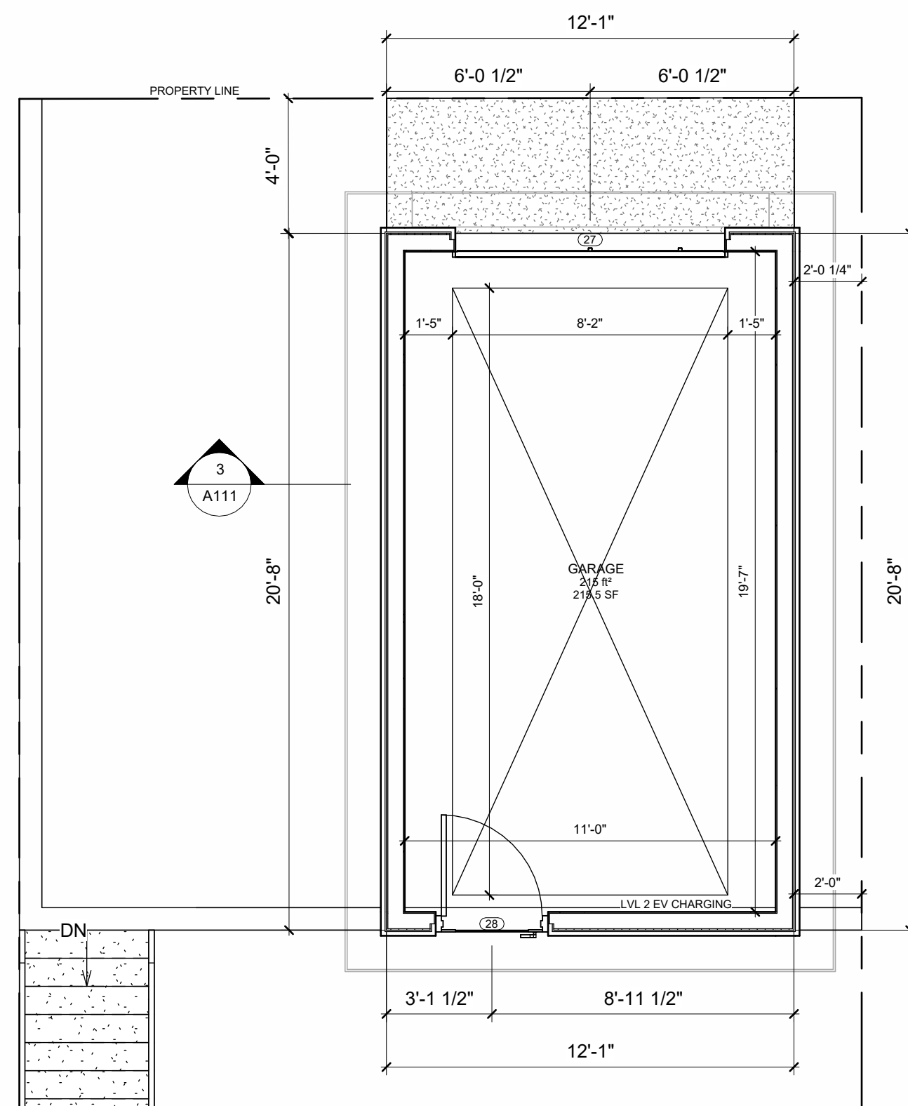
1 GARAGE FLOOR PLAN 1/4" = 1'-0"
