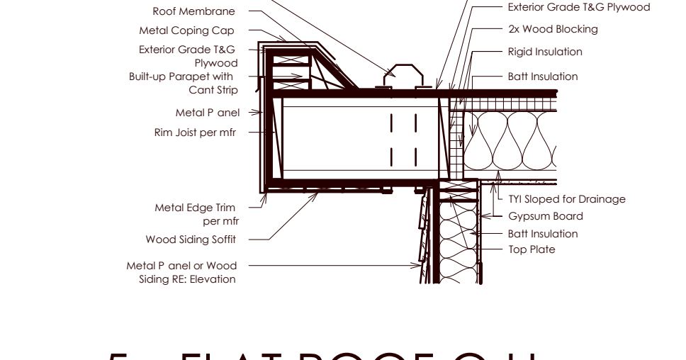
5 FLAT ROOF O.H
