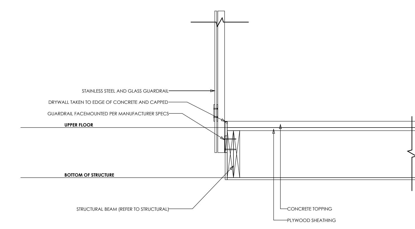
10 GUARDRAIL 1" = 1'-0"
