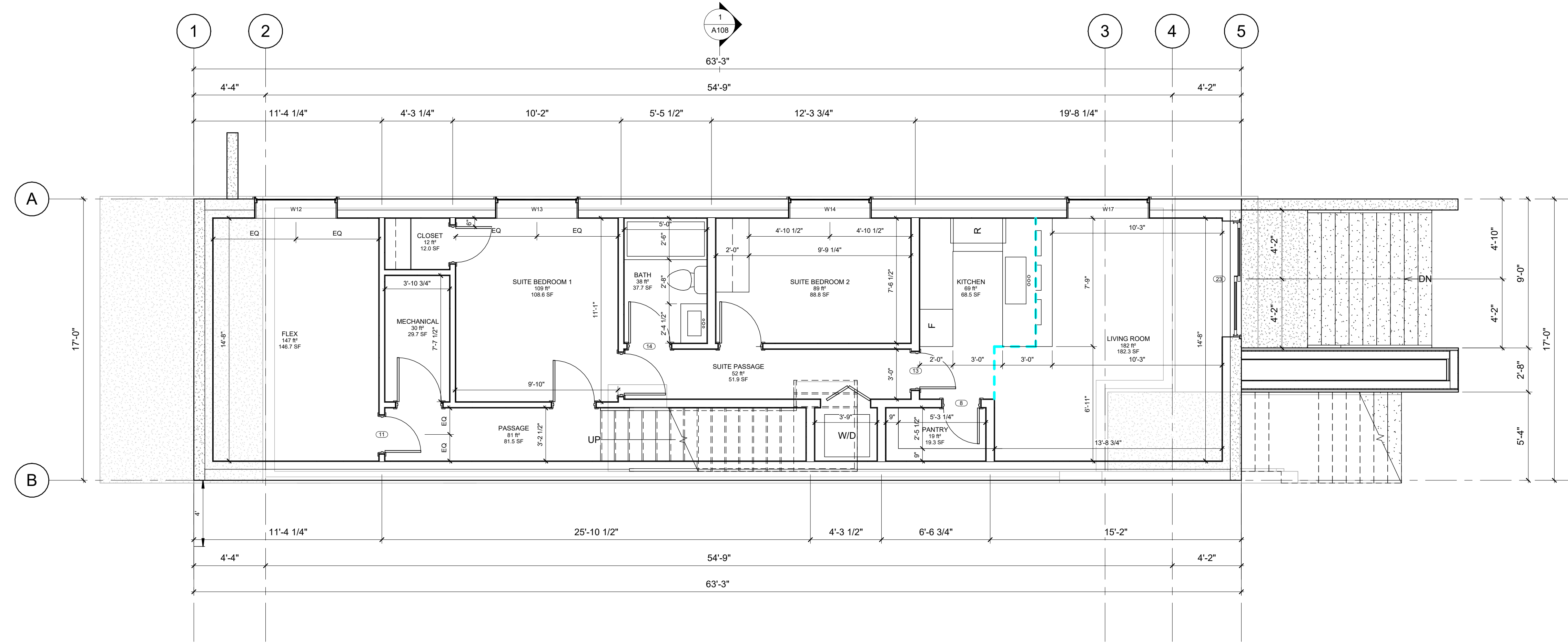
1 BASEMENT 1/4" = 1'-0"
