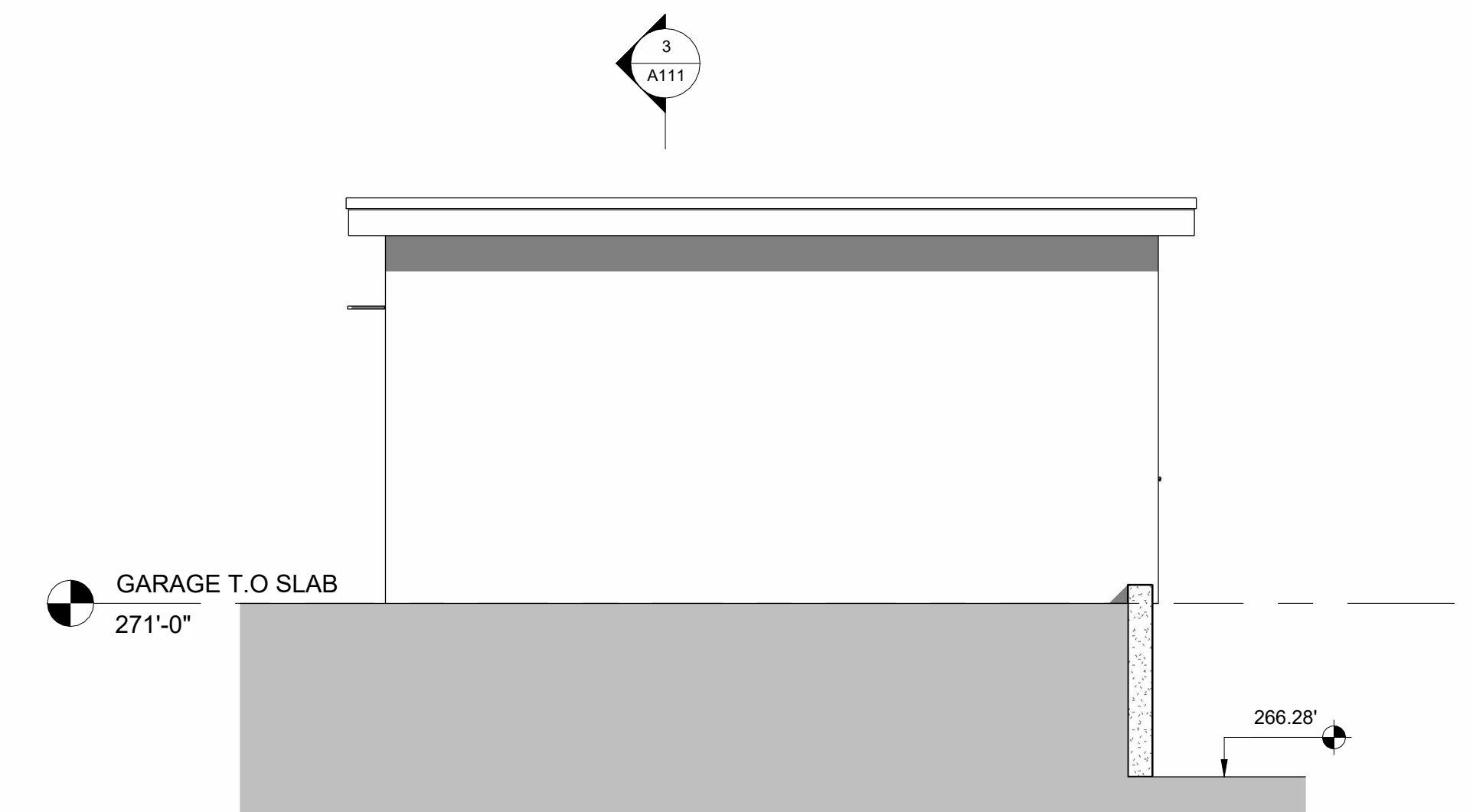
7 GARAGE - WEST 1/4" = 1'-0"
