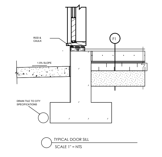
4 TYPICAL DOOR SILL SCALE 1" = 1/4"
