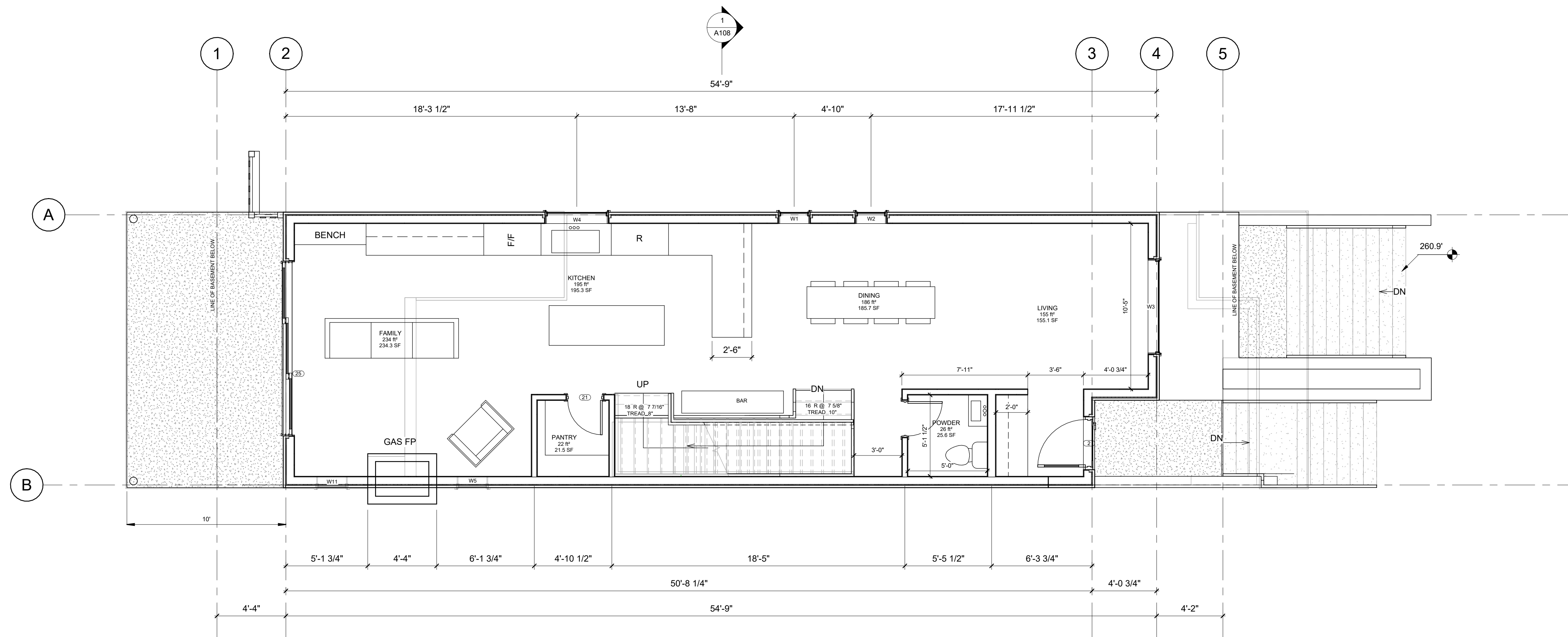
1 MAIN FLOOR 1/4" = 1'-0"
