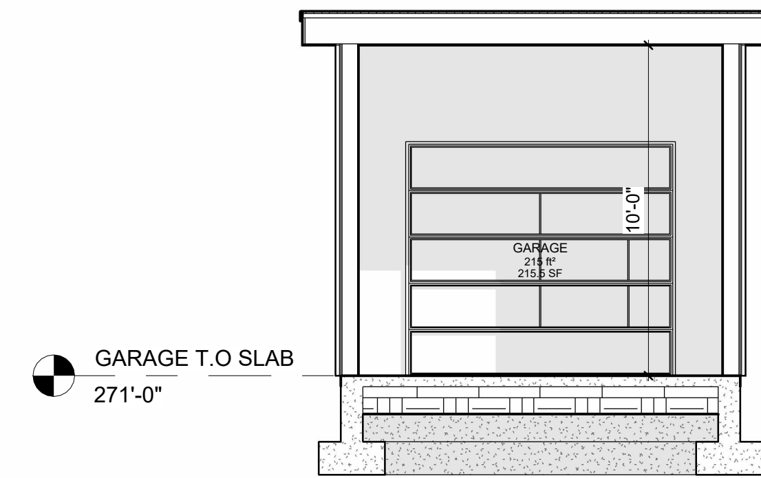
3 GARAGE SECTION 1/4" = 1'-0"
