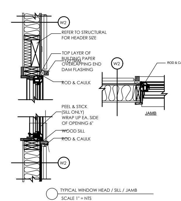
1 TYPICAL WINDOW HEAD / SILL / JAMB SCALE 1" = 1/4"
